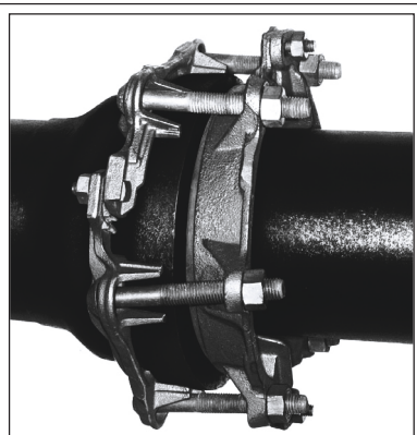
For repair of cast iron bell & spigot joints
