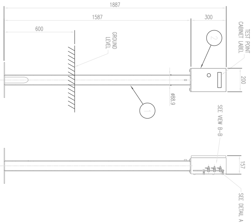
DN80 TEST POINT UPSTAND & ALUMINIUM ENCLOSURE SCALE 1:15
